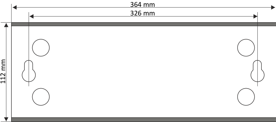
Case dimensions and distances between mounting holes - rear view
