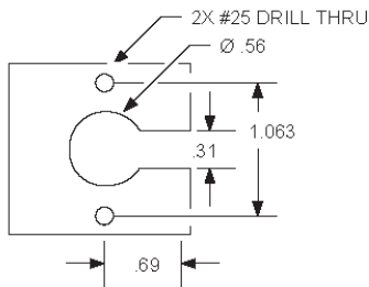
Recommended Mounting Plate Dimensions
