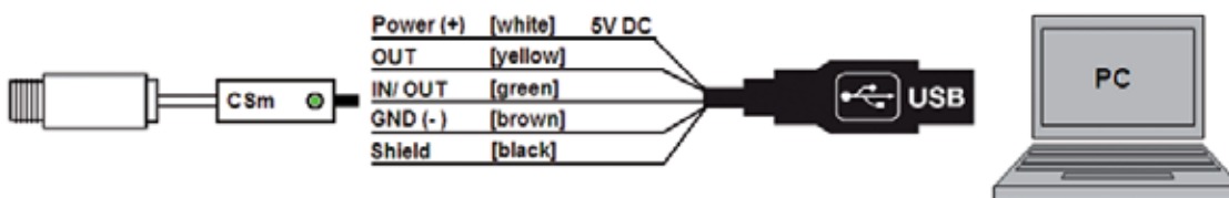
Connection digital with USB adapter cable
