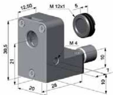
Air purge collar with integrated CF-lens (ACCTAPLCF)
