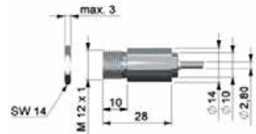
Dimensions optiris CSmicro LT
