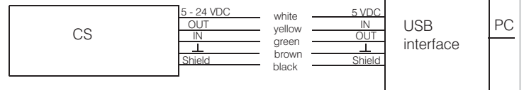
Connection diagram CS/USB programming interface
